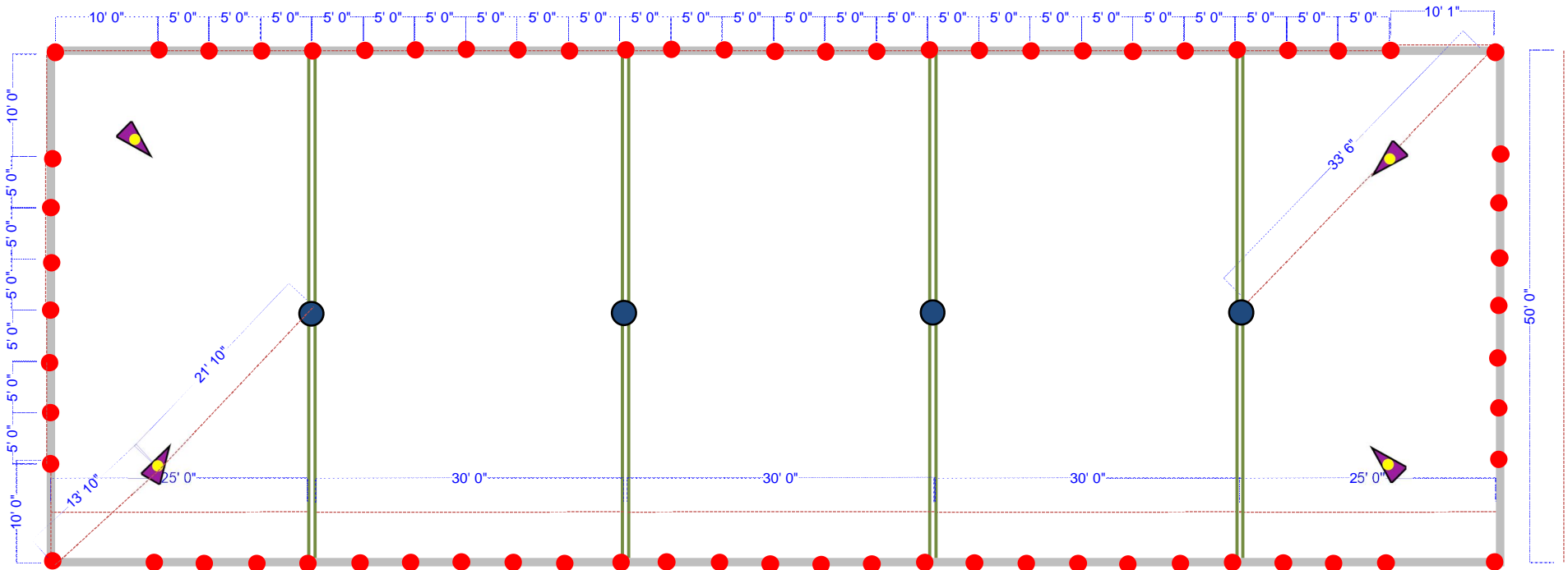
50' x 140' Pole Tent - Pole Placements
